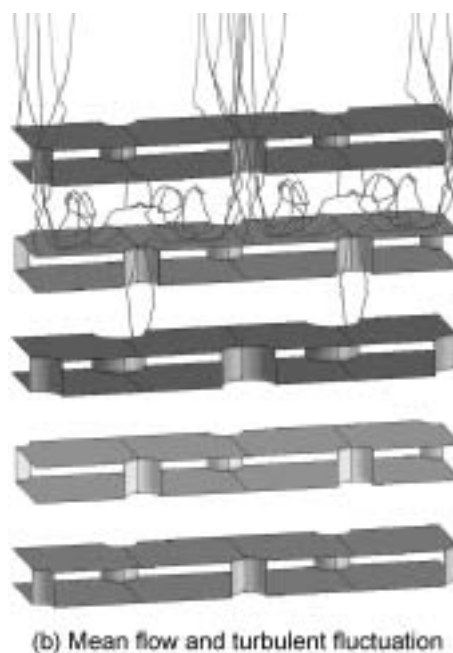
Fig. 6. Particle trajectory of 5 stage system ( d_p: 1 \mu\text{m} , v_{s,in}: 1.0 m/s, plate arrangement: [2, 2, 3, 2, 2 mm]).
