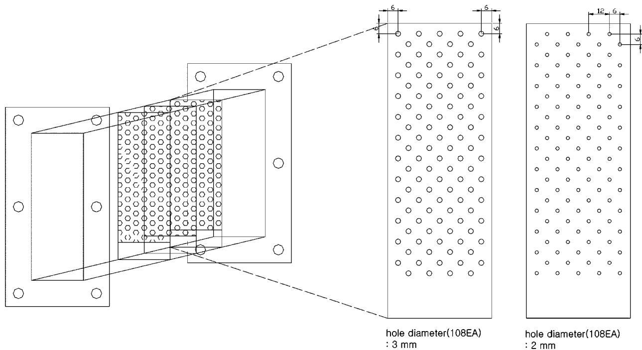
Fig. 2. Configuration of multi-stage porous plate.
